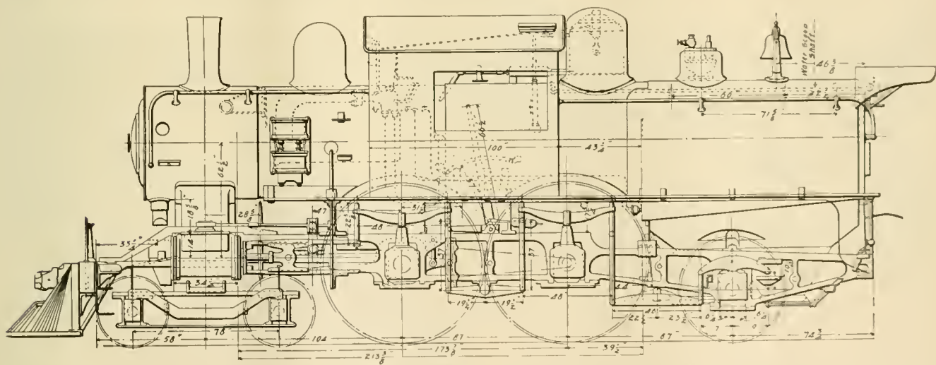
ATLANTIC LOCOMOTIVE ELEVATION-CENTRAL RAILROAD OF NEW JERSEY.
